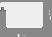
Wandprofil Wall profile
